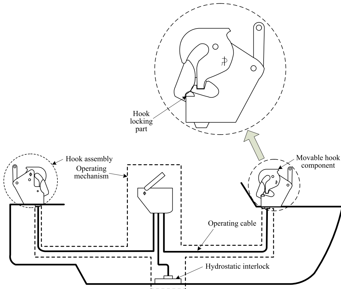
Lifeboat release and retrieval system
